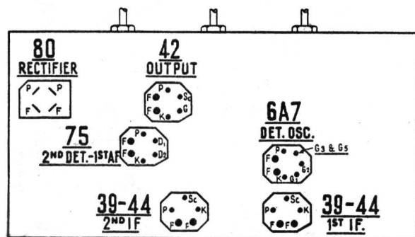
Fig. 1—Tube Socket Layout (underside)
