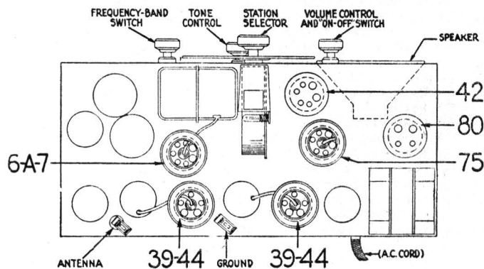
Fig. 2—Chassis Top View
